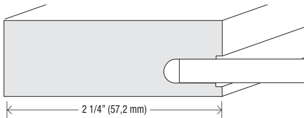
Battant Rail
